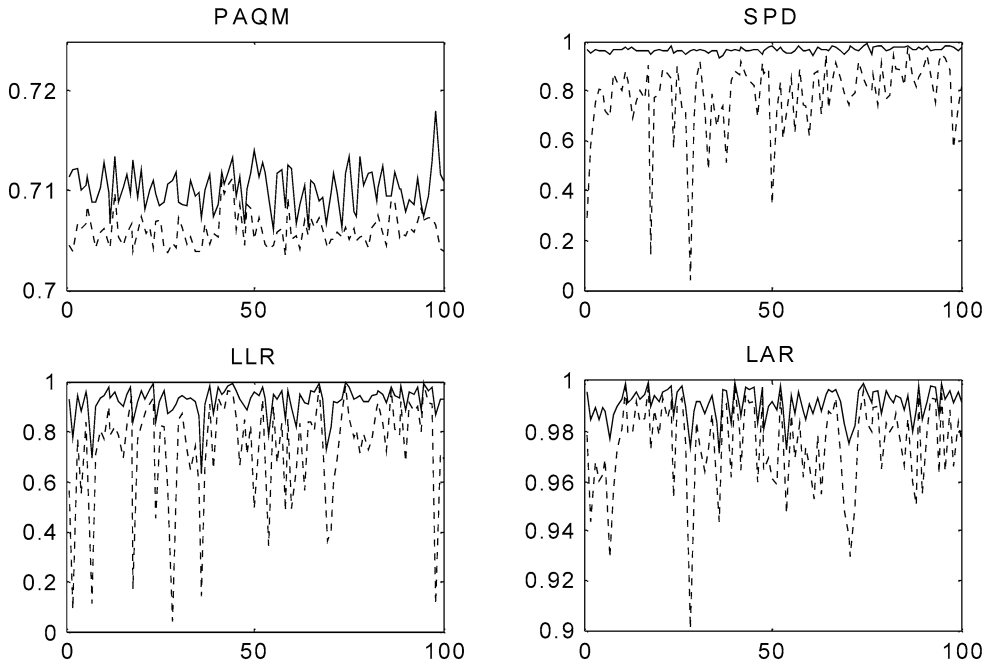
Fig. 2. Four distance metrics calculated from 100 utterances, the dotted lines are distance measures evaluated from stego-objects and the solid lines are from the cover objects. The abscissa denotes the index of utterances.
