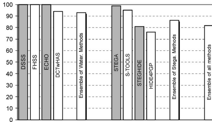
Fig. 3. Bar charts of the correct detection performance of the steganalyzer.
