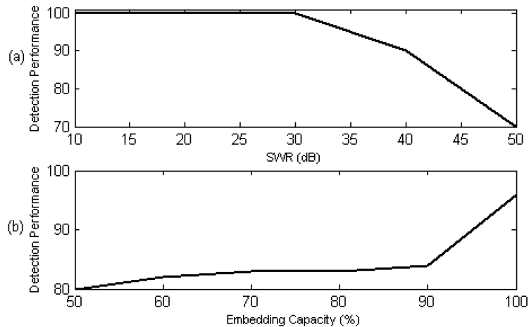
Fig. 4. (a) Dependence of steganalysis performance on the DSSS watermarking strength. (b) Dependence of steganalysis performance on the embedding capacity of the S-tools steganographic method.
