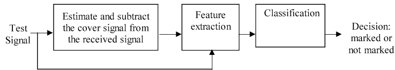
Fig. 1. Block diagram of the steganalysis method.
